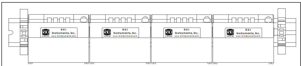
Figure 8: 4-Charger Installation
