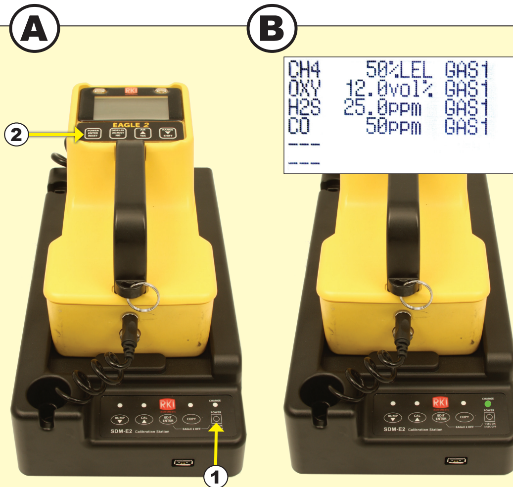
Instrument Connected
