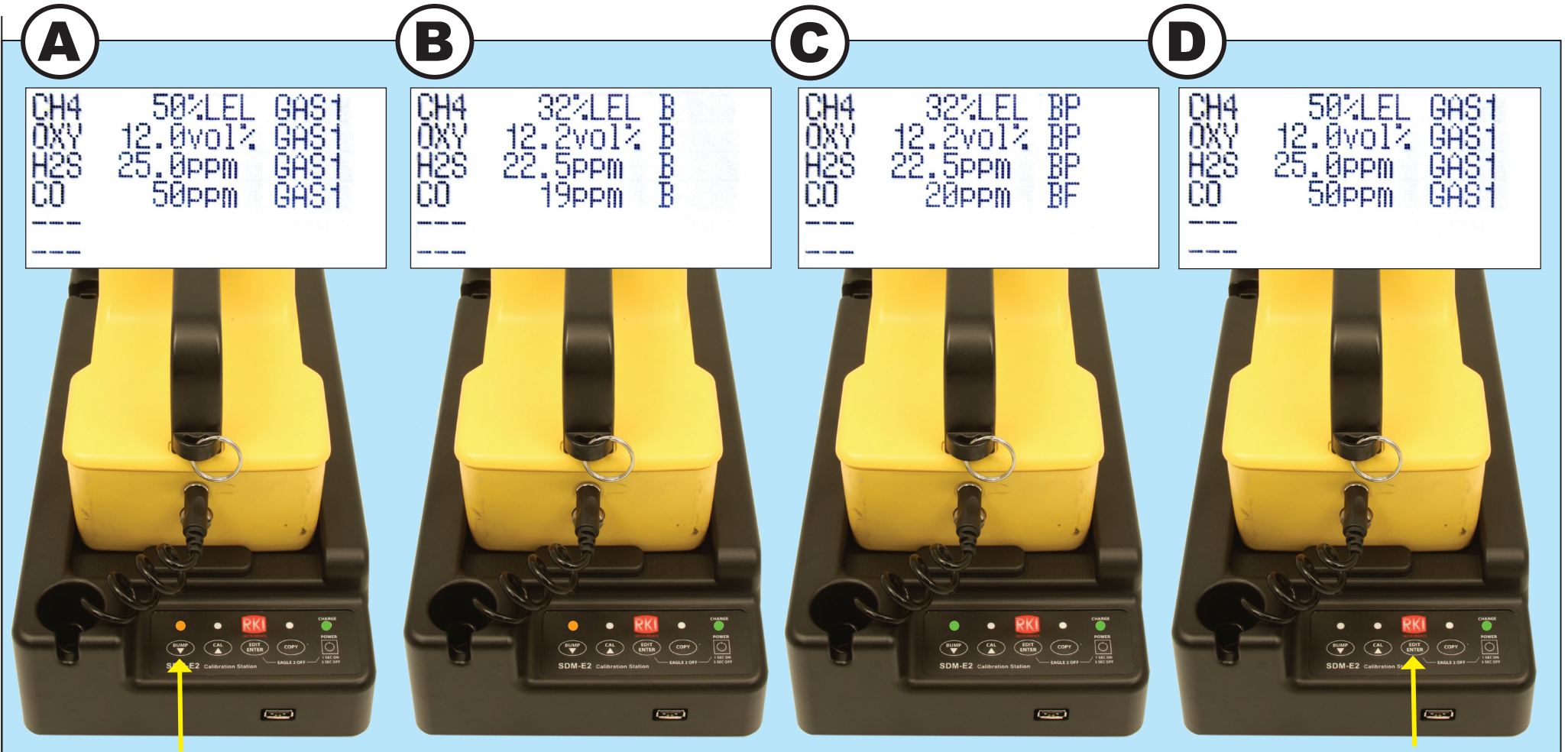
Bump Test
