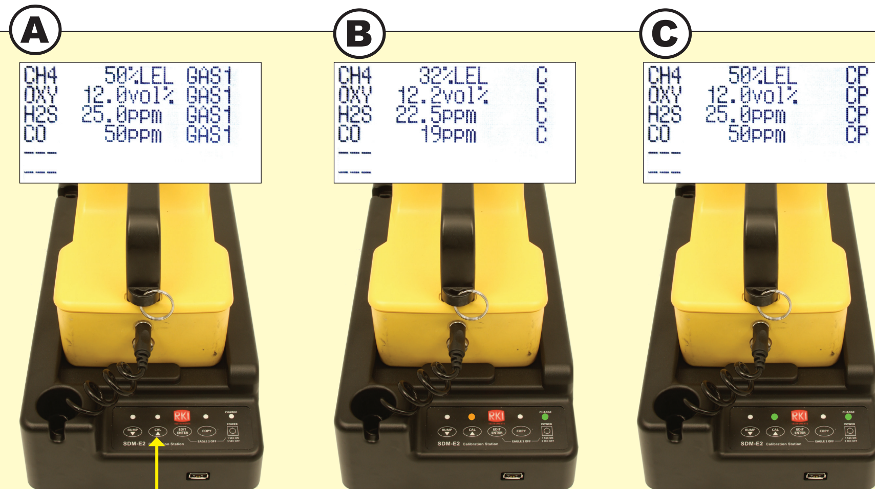
Calibration Results
