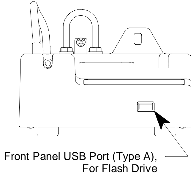
Figure 9: Front Panel
