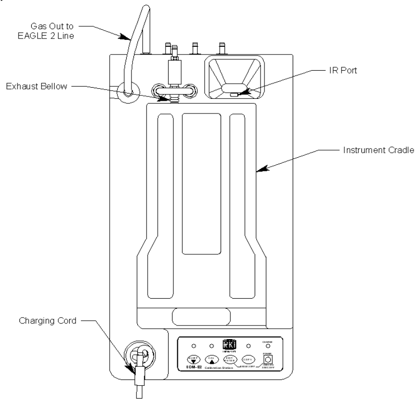
Figure 6: Instrument Panel
