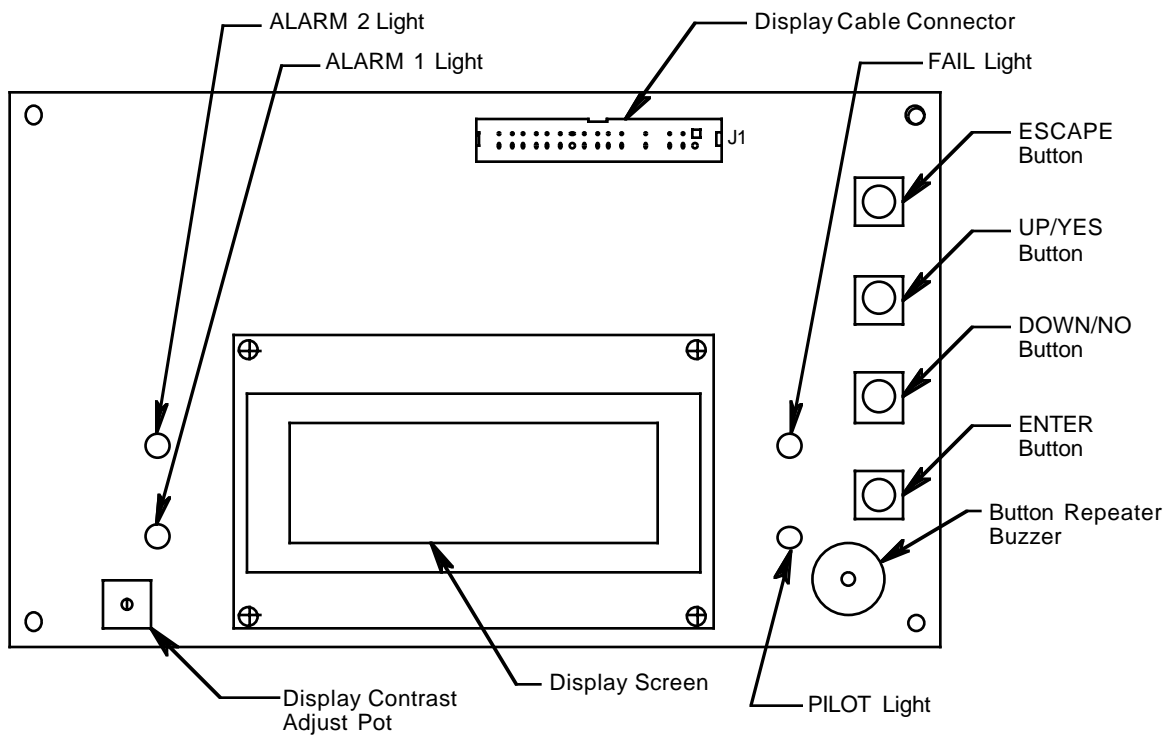
Figure 2. Display Board Component Location
