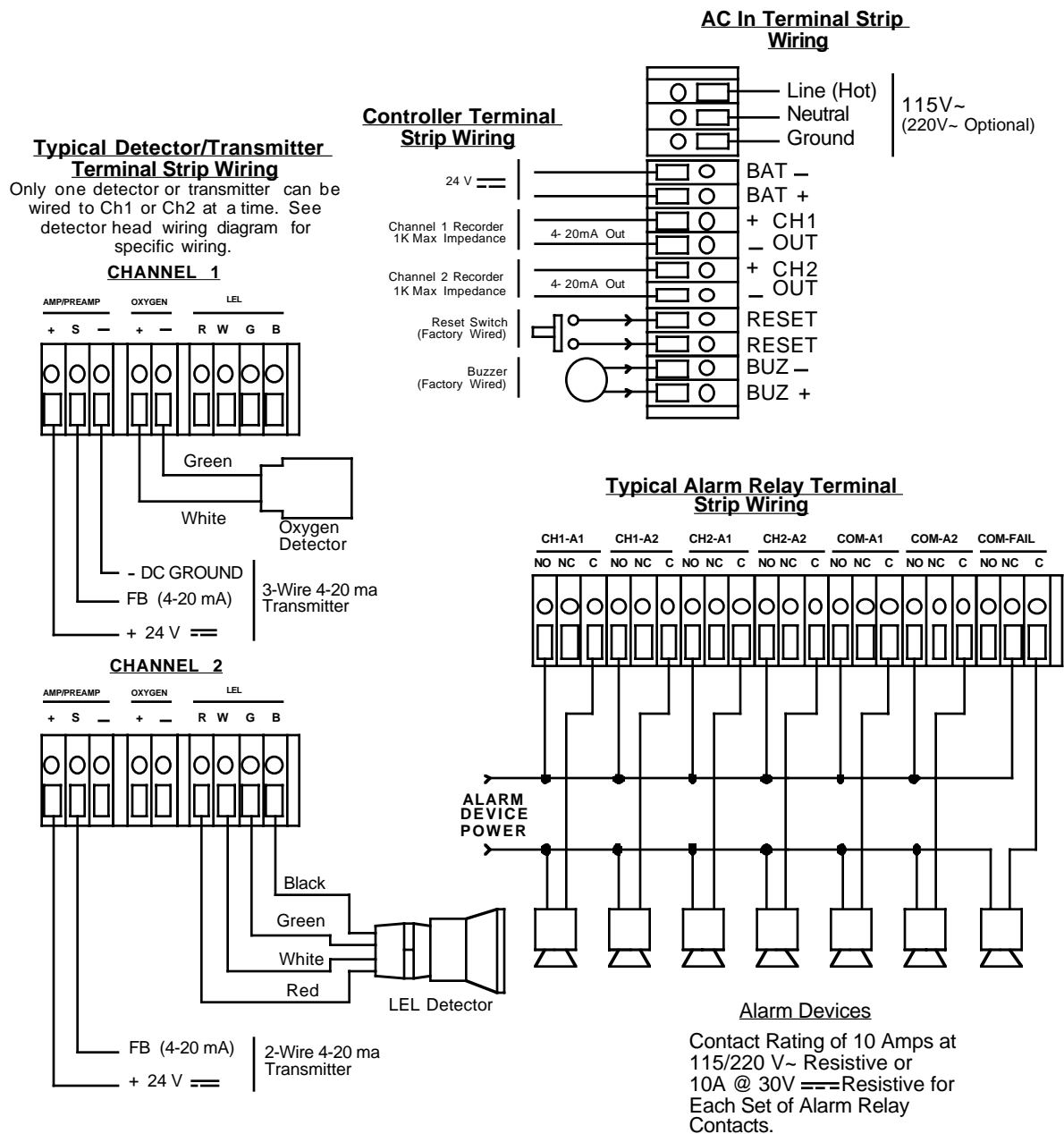
Figure 5. Beacon 200 Gas Monitor General External Wiring Diagram
